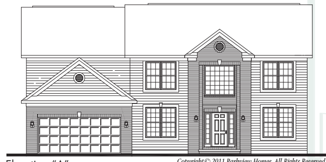
Elevation "A" Copyright © 2011 Parkview Homes, All Rights Reserved.
