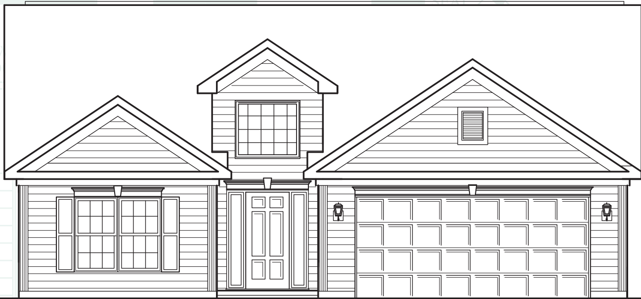
Elevation "O"
